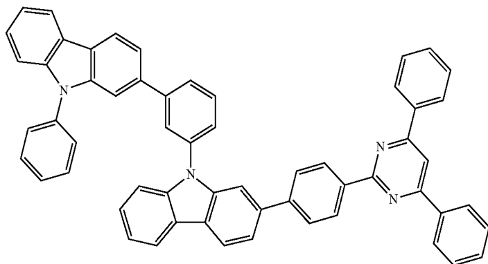
Chemical Formula 1-32
