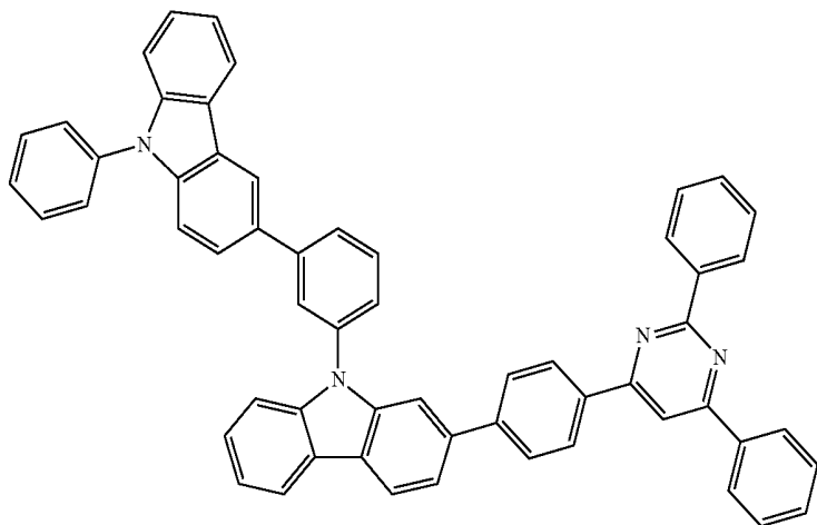
Chemical Formula 1-25
