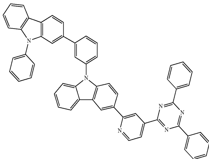
Chemical Formula 1-119
