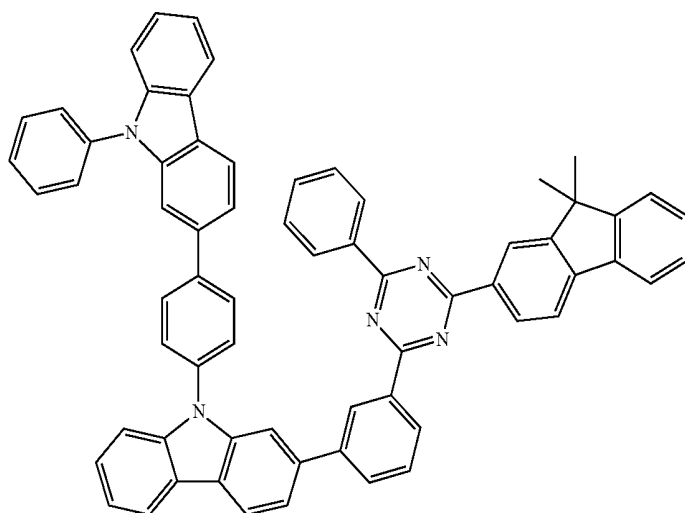
Chemical Formula 1-212
