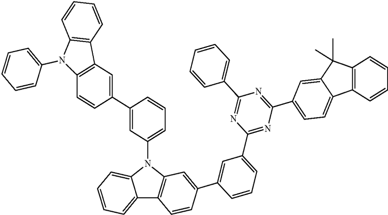
Chemical Formula 1-208
