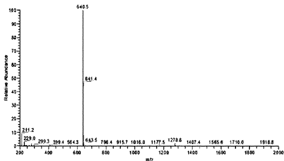
Mass spectrum of chemical Formula 1-227
