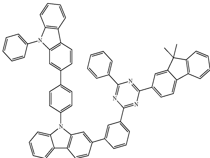
Chemical Formula 1-212
