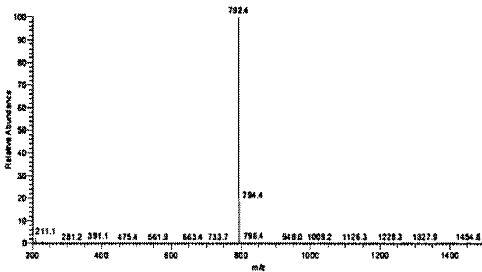
Mass spectrum of chemical Formula 1-4
