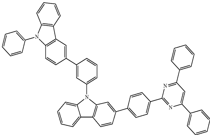
Chemical Formula 1-31
