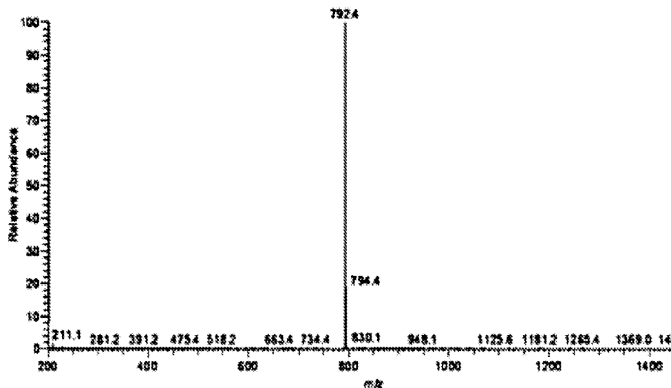
Mass spectrum of chemical Formula 1-5
