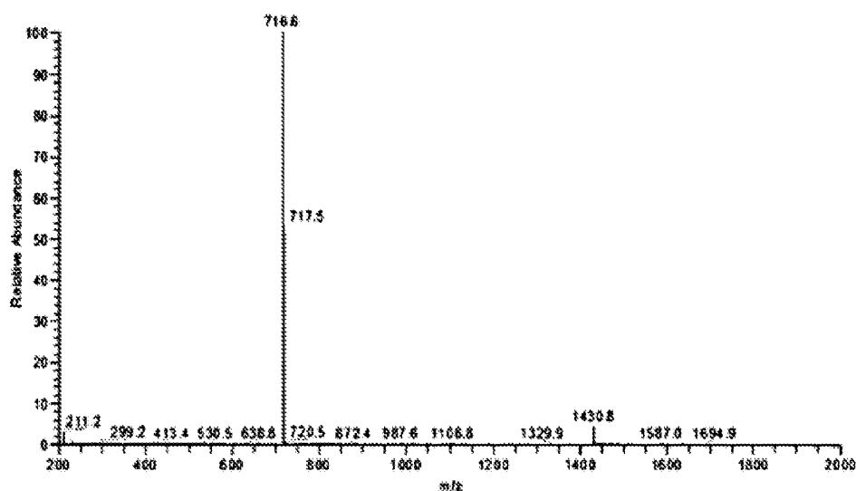
Mass spectrum of chemical Formula 1-228
