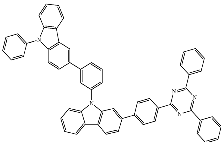
Chemical Formula 1-19
