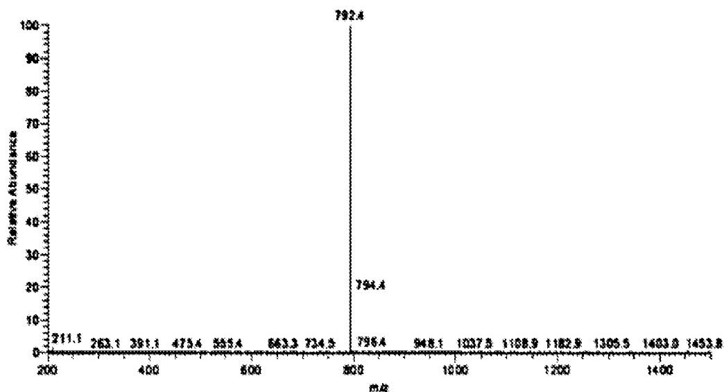
Mass spectrum of chemical Formula 1-71
