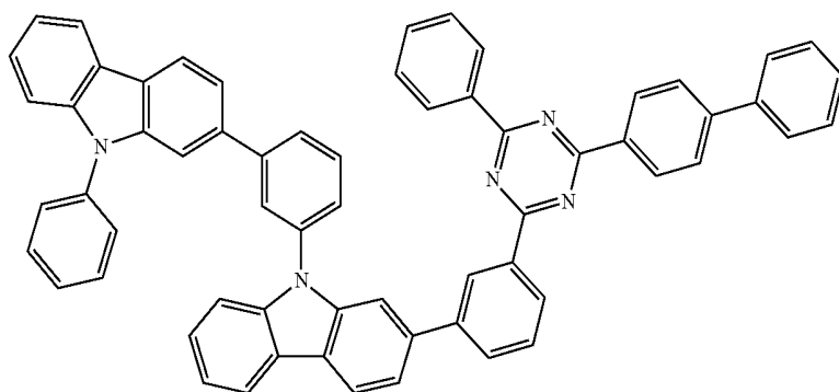
Chemical Formula 1-13
