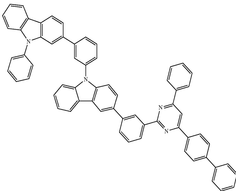
Chemical Formula 1-83
