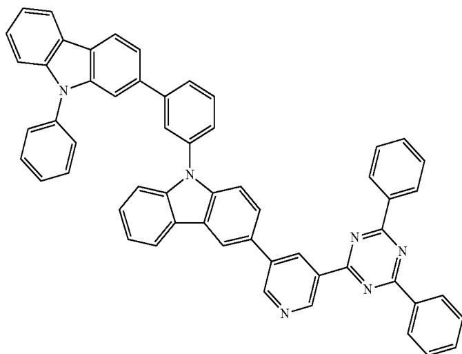
Chemical Formula 1-107
