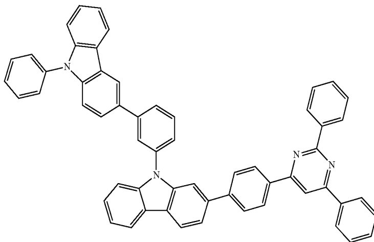
Chemical Formula 1-25
