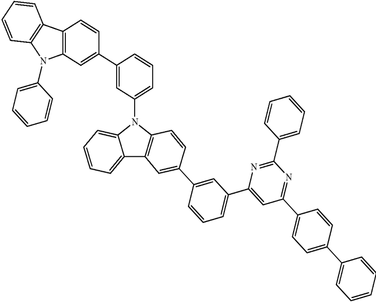
Chemical Formula 1-84
