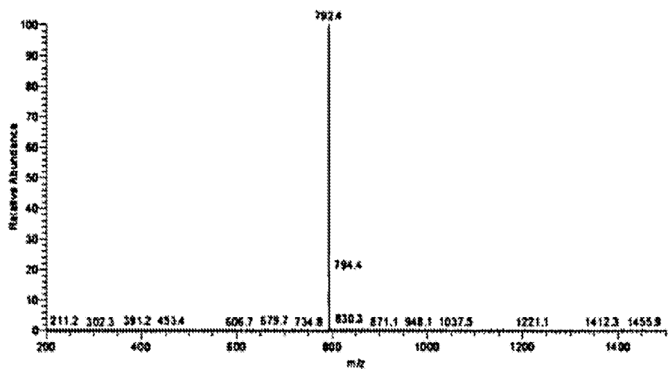
Mass spectrum of chemical Formula 1-142
