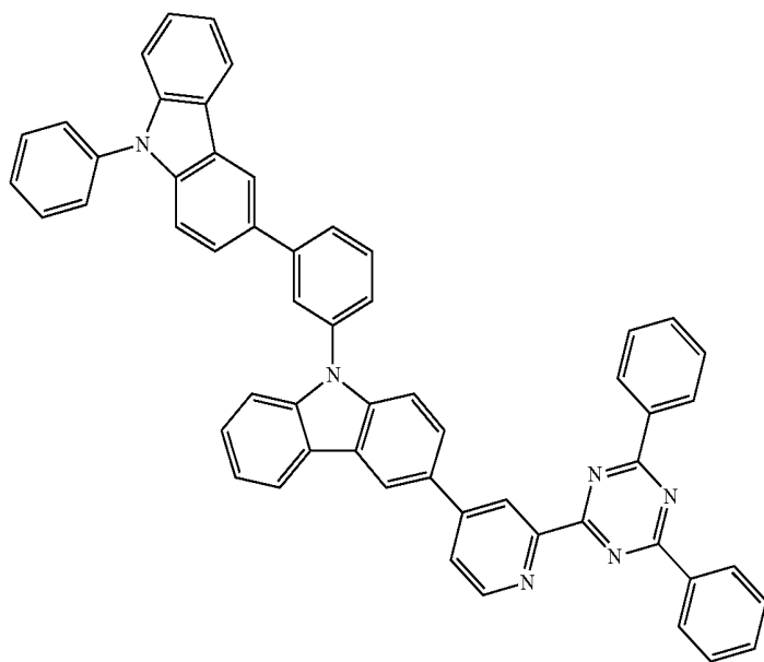
Chemical Formula 1-112
