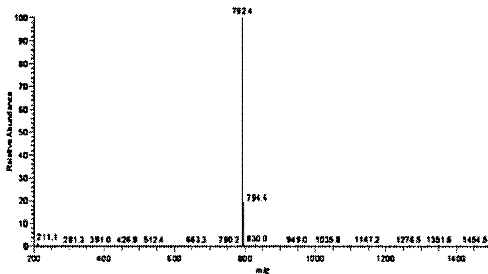
Mass spectrum of chemical Formula 1-23
