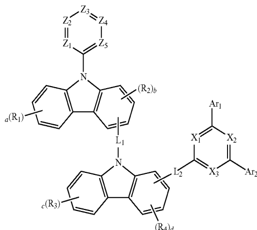
[Chemical Formula 2]
