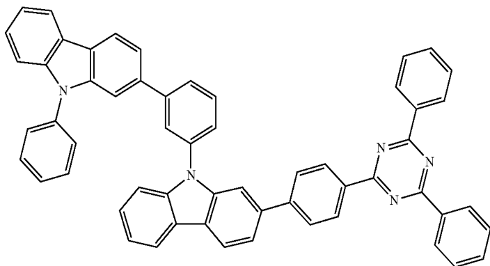
Chemical Formula 1-20
