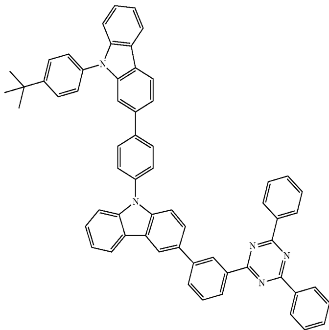
Chemical Formula 1-134
