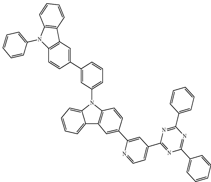
Chemical Formula 1-118
