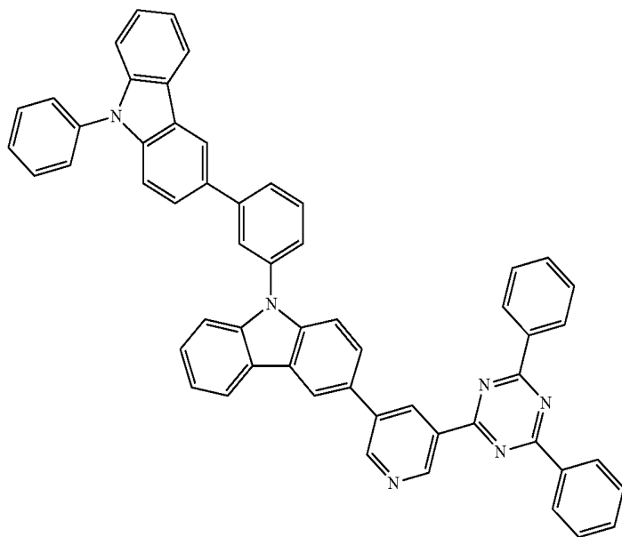
Chemical Formula 1-106
