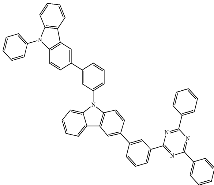
Chemical Formula 1-70
