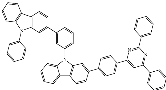
Chemical Formula 1-26
