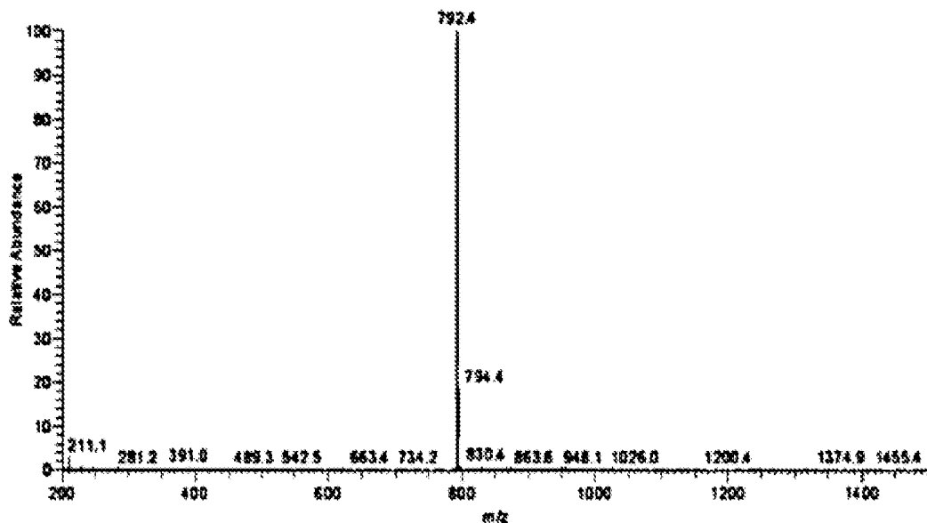
Mass spectrum of chemical Formula 1-70
