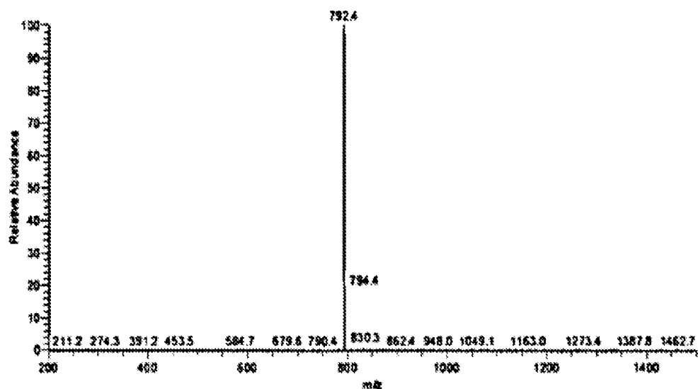
Mass spectrum of chemical Formula 1-2
