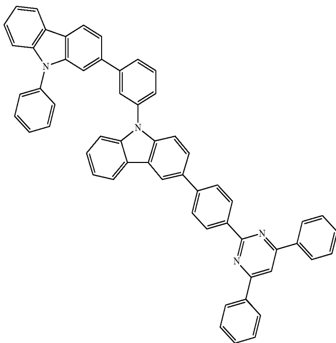
Chemical Formula 1-101
