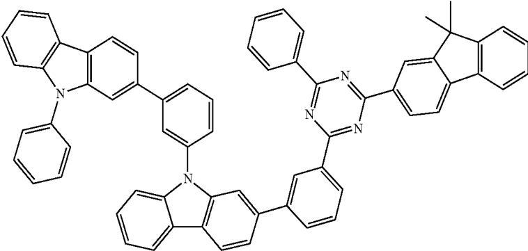
Chemical Formula 1-209
