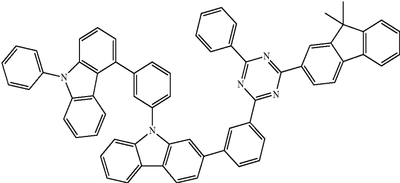
Chemical Formula 1-210
