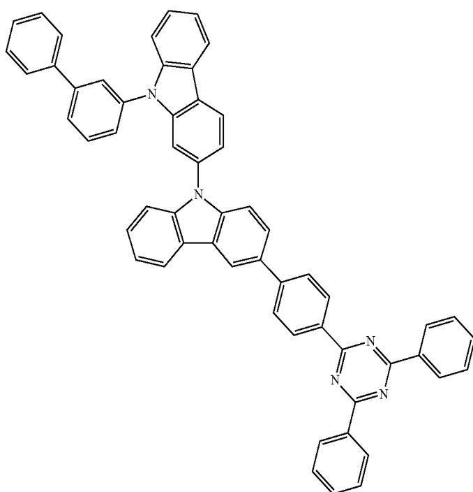
Chemical Formula 1-230
