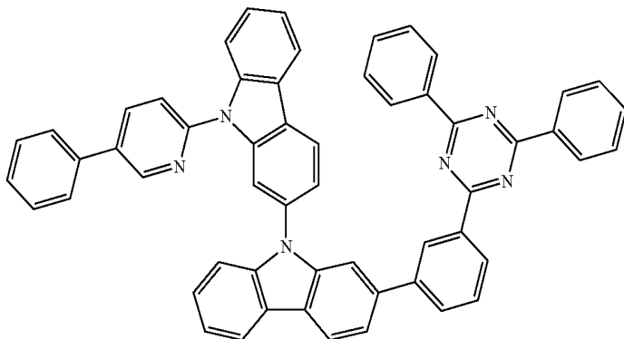
Chemical Formula 1-231
