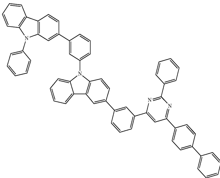
Chemical Formula 1-84
