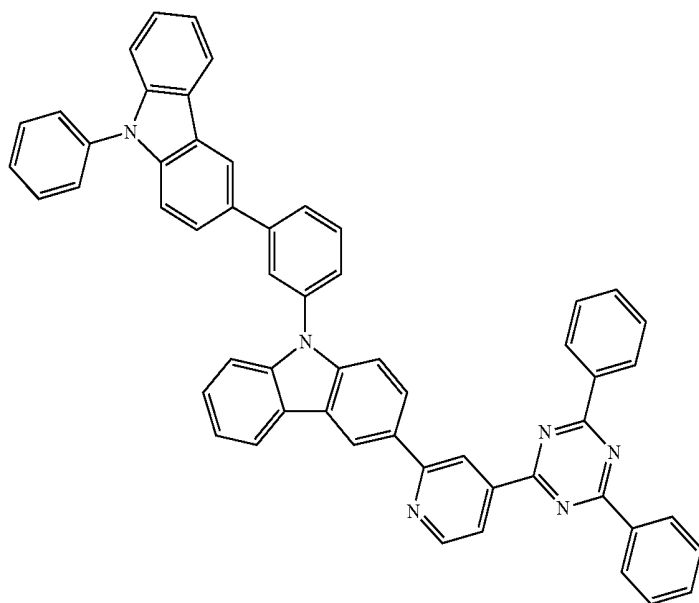
Chemical Formula 1-118
