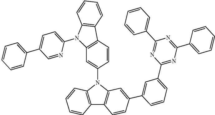
Chemical Formula 1-231
