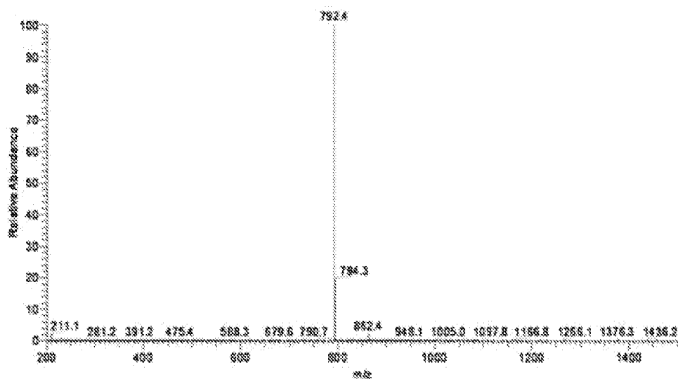
Mass spectrum of chemical Formula 1-1
