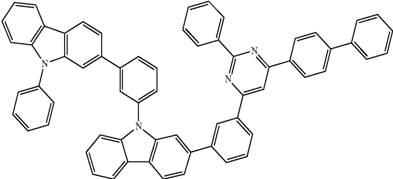
Chemical Formula 1-15
