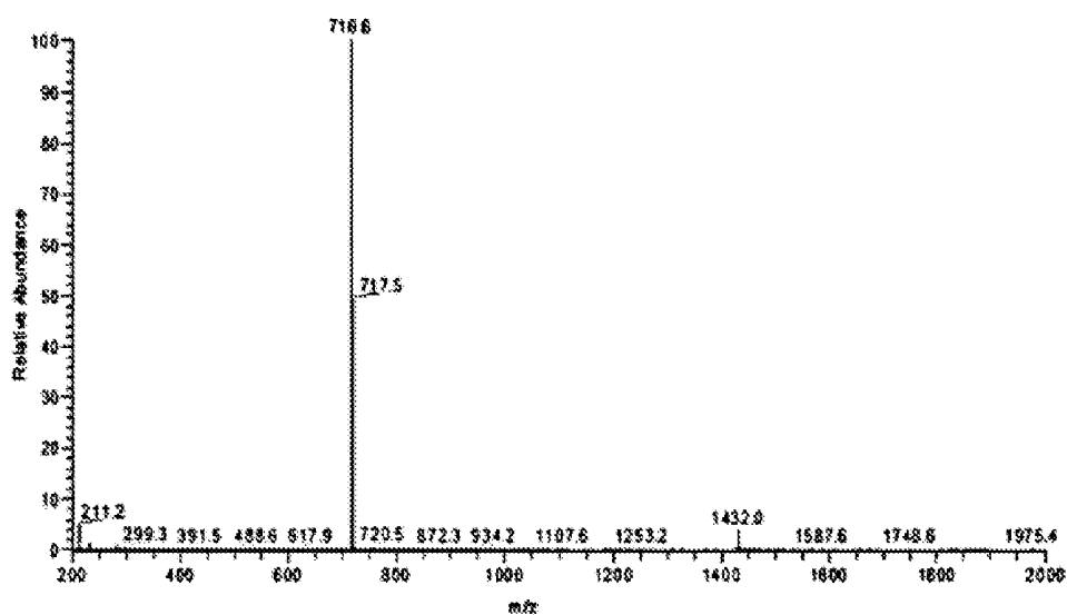
Mass spectrum of chemical Formula 1-219
