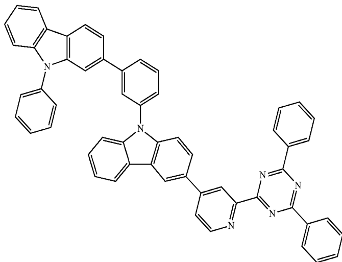
Chemical Formula 1-113
