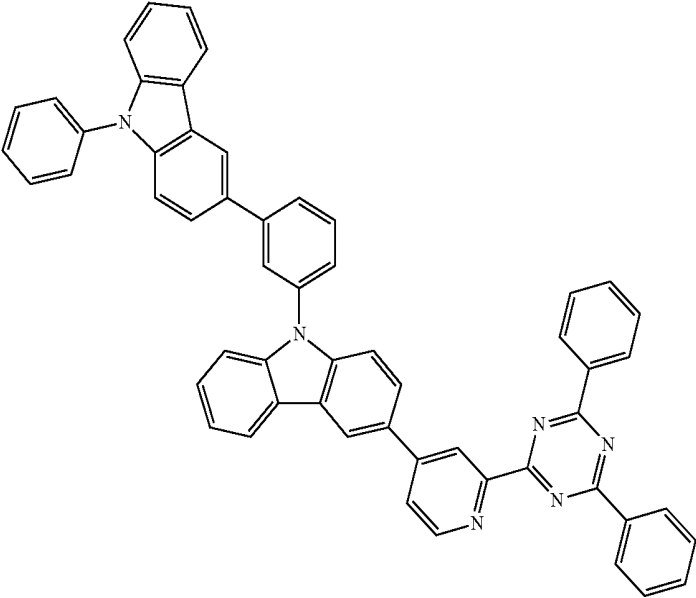
Chemical Formula 1-112
