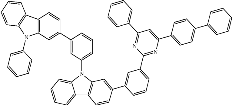
Chemical Formula 1-14
