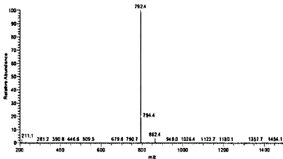
Mass spectrum of chemical Formula 1-19
