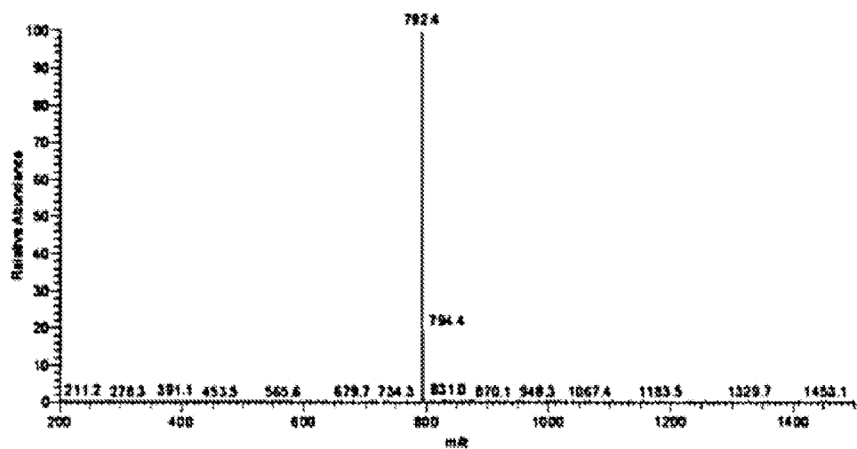
Mass spectrum of chemical Formula 1-74
