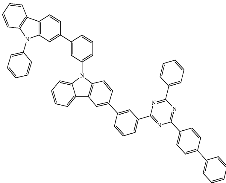
Chemical Formula 1-82
