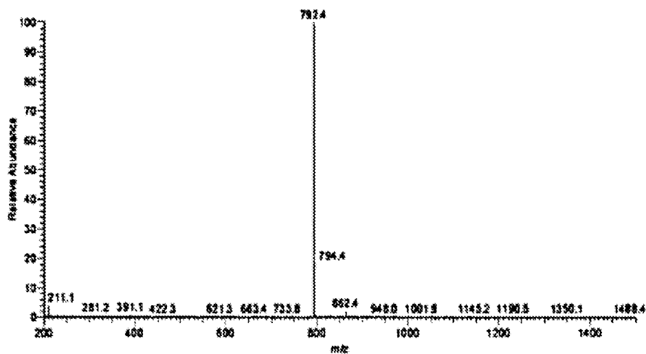
Mass spectrum of chemical Formula 1-160
