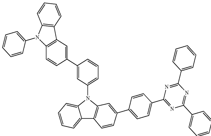
Chemical Formula 1-19
